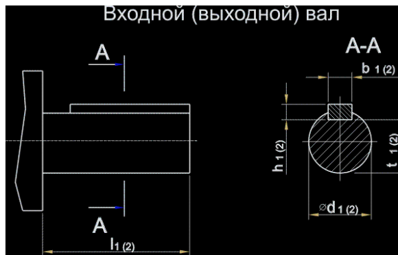
Overall and mounting dimensions
