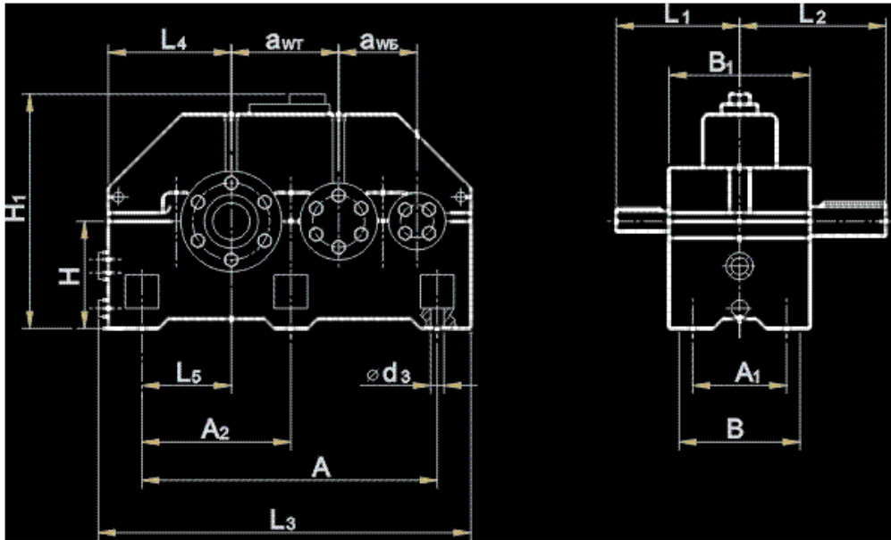
Overall and mounting dimensions
